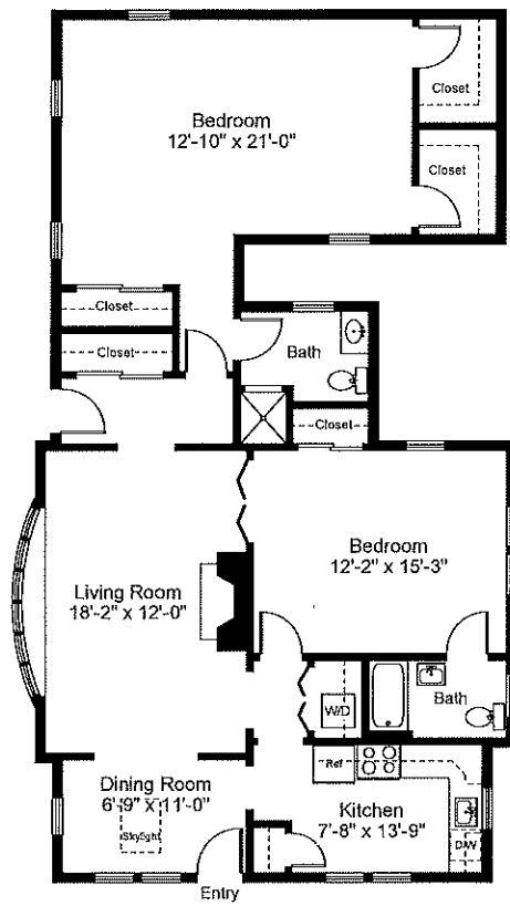
Cottage Floor Plan Ceiling Height = 7'-8"
